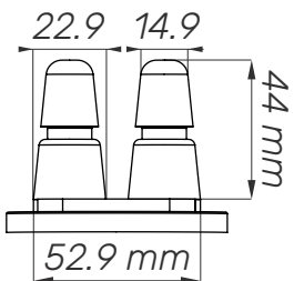
Double pin mount
